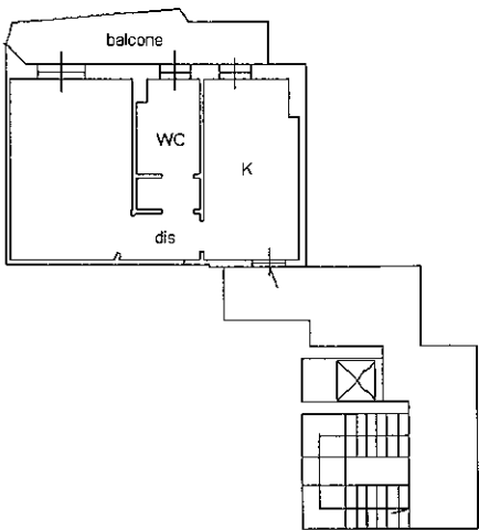
PIANO SESTO H 290
